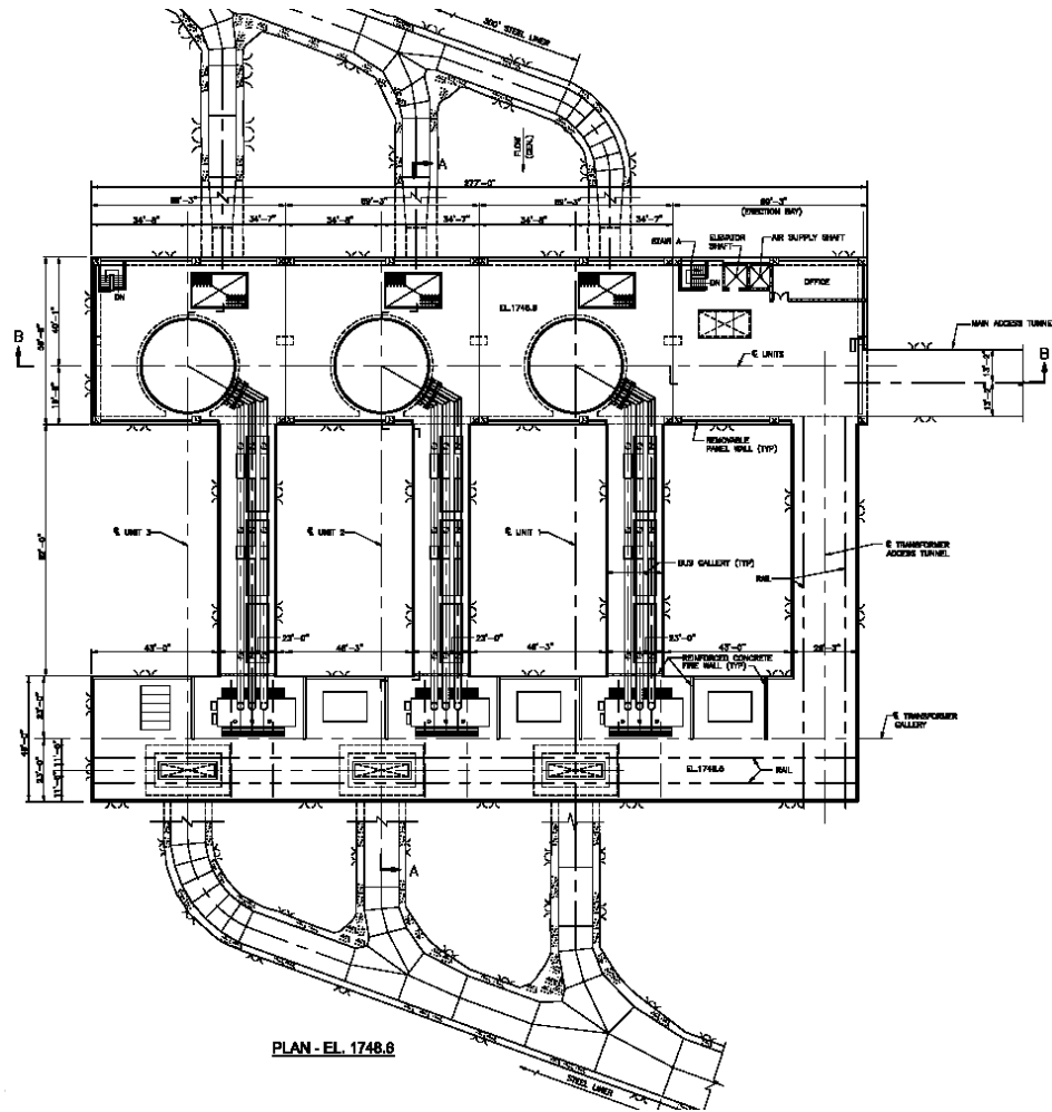
Figure 5.2-3 Powerhouse Plan View at Elevation 1748.8 ft.
