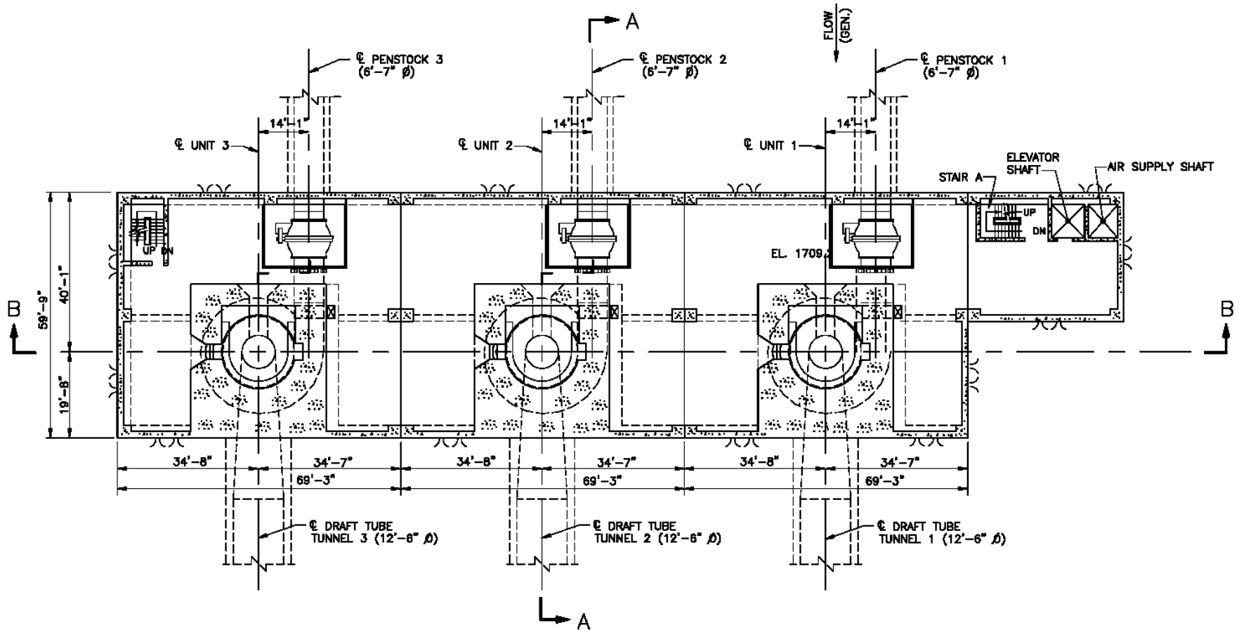
PLAN - EL. 1709.2
