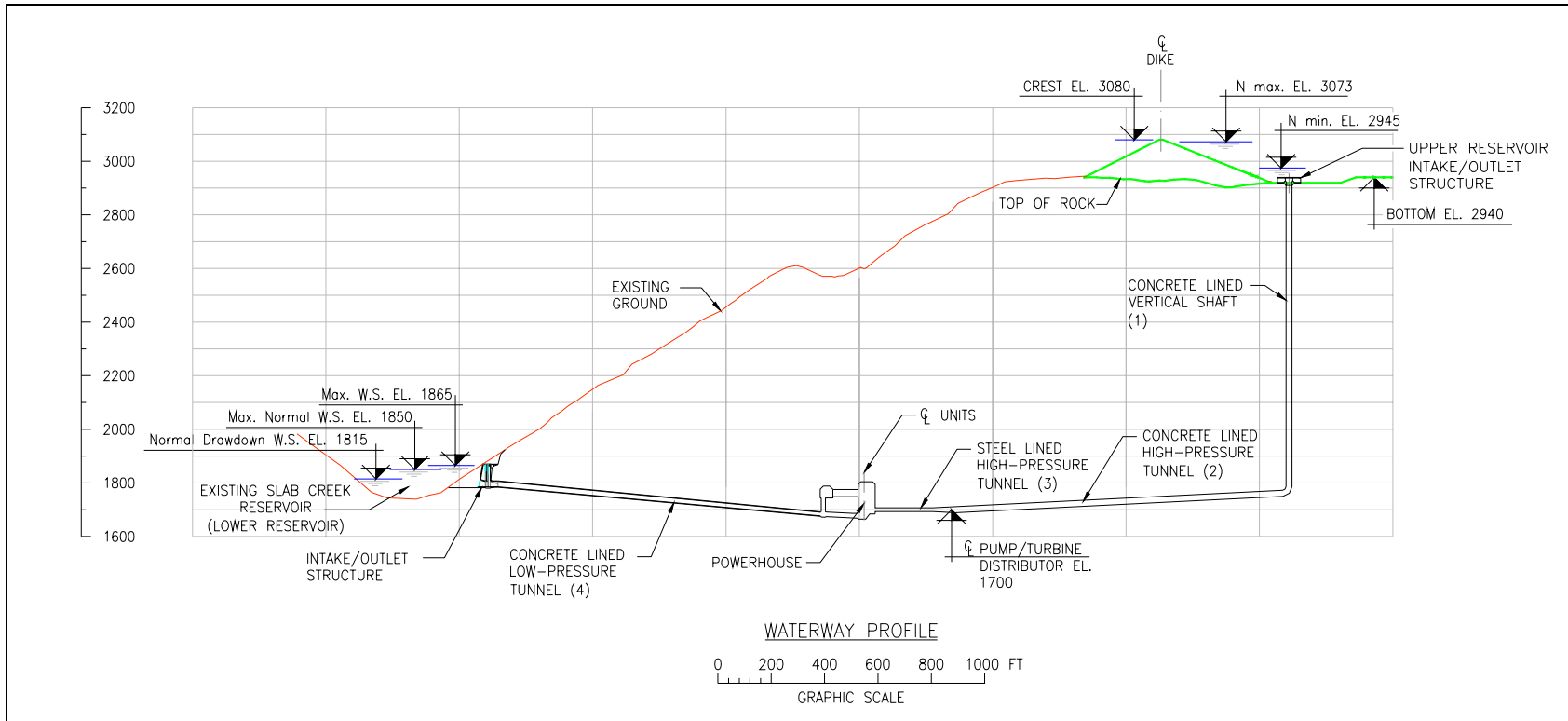
Figure 5.1 Cross-Section of Iowa Hill Pumped Storage Development
