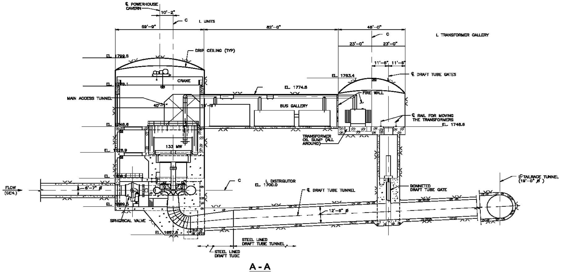
Figure 5.2-2 Powerhouse Cross-Section View 2
