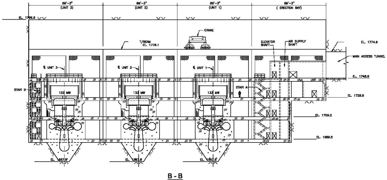
Figure 5.2-1 Powerhouse Cross-Section View 1
